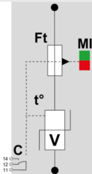
V: High-energy varistor Ft: Thermal fuse C: Remote signal contact t°: Thermal disconnection system MI: Disconnection indicator
