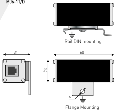
MJ6-1T/D
