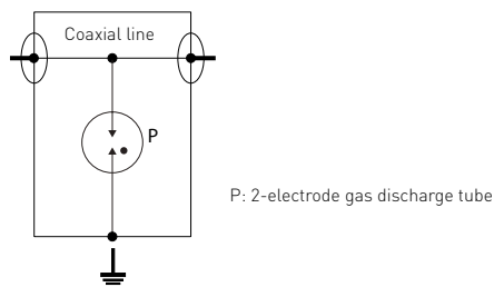
P8AX_-B/FF
