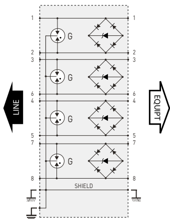
G: 3-electrode gas tube
