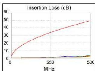
TRANSMISSION CURVES (MJ8-C6A)
