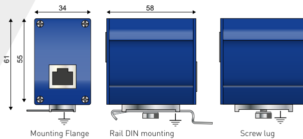
Mounting Flange
