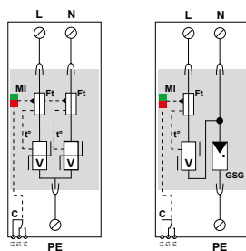
DAC40CS-20 DAC40CS-11
