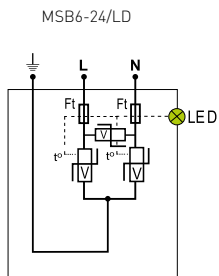
MSB6-24/LD
