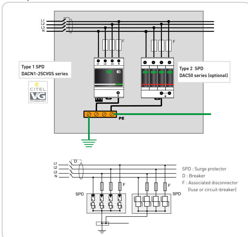
Example of coordination on 3-Phase network
