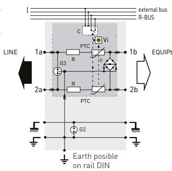
DLAWTS1-xxx DLAWTS1-xxx/R Line cut-off if plugout
