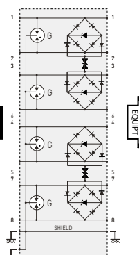
MJ8-POE-C6A
