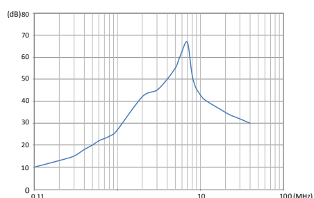
Attenuation curve
