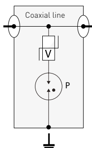
V: Varistor P: 2-electrode gas tube
