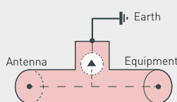
P8AX / P8AX-6G
