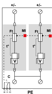
DS72RS-48DC
