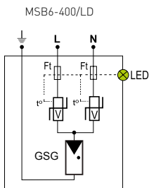
MSB6-400/LD
