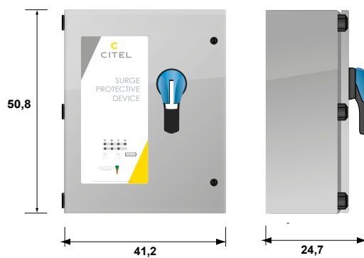
MDS750E series
