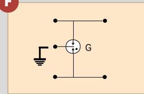
F 3-electrode GDT Protection
