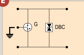
E High bit-rate Protection
