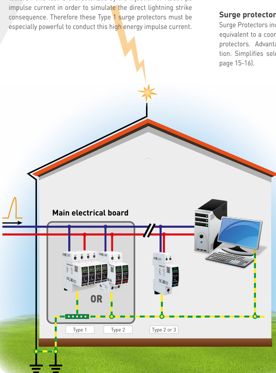
Different SPD types following IEC and EN standards
