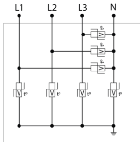
V: High-energy varistor t*: Thermal disconnection system
